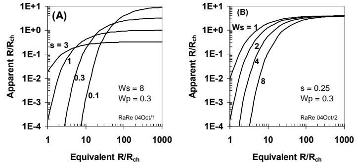
Fig. 3. Numerical examples of R_{ap} vs. R_{eq}
