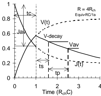
Fig.2. Time relations of measured current and voltage with scanning charger and probe.
