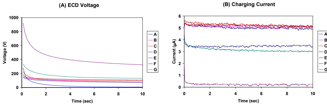
Fig. 7 (A) Voltage and (B) Charging Current as a function of time for 7 intermediate transfer belt samples.
