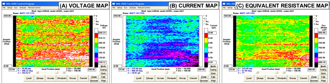
Fig. 6 (A) Voltage, (B) Current, and (C) Equivalent Resistance Maps for the same sample in Fig. 5.
