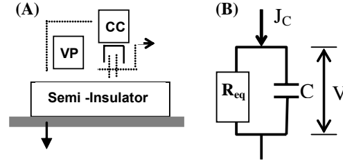
Fig. 1. (A) Schematic of ECD experimental setup, with corona charger (CC) and voltage probe (VP); (B) Equivalent circuit for the sample.
