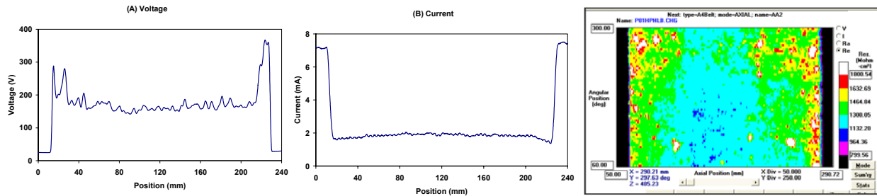
Fig. 8 (A) Voltage, (B) Current and (C) Equivalent Resistance Map for an electrophotographic paper sample.
